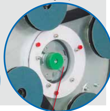
Gear protection against dust and slurry
